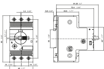
MBS32NH ≤ 10 A
