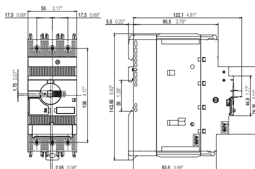
MBS63NH
